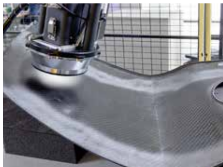
F-SCAN sensor scanning carbon composite part
