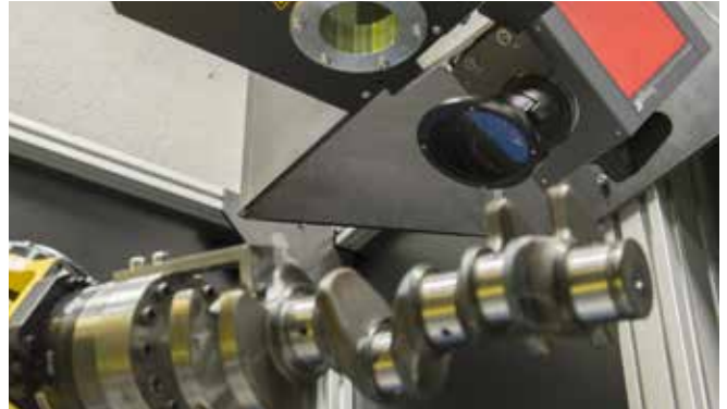
Industrial thermography: automated non-destructive crack detection
